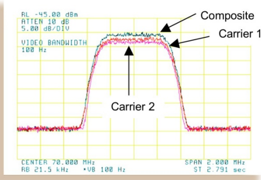
Figure 2: Duplex Link with DoubleTalk Carrier-in-Carrier
